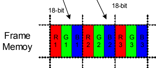
Look-Up Table for 65k Colors mapping (16-bit to 18-bit)
